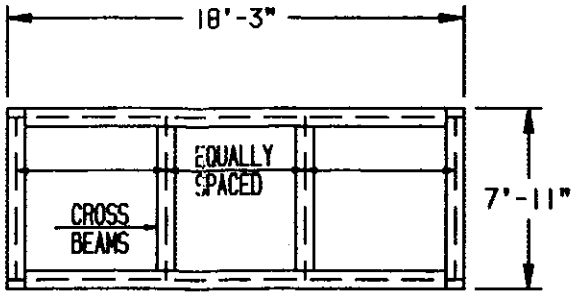
TYPICAL PLAN OF SUPPORT SIZE OF BEAMS ACCORDING TO OPERATING WEIGHT OF UNIT.
