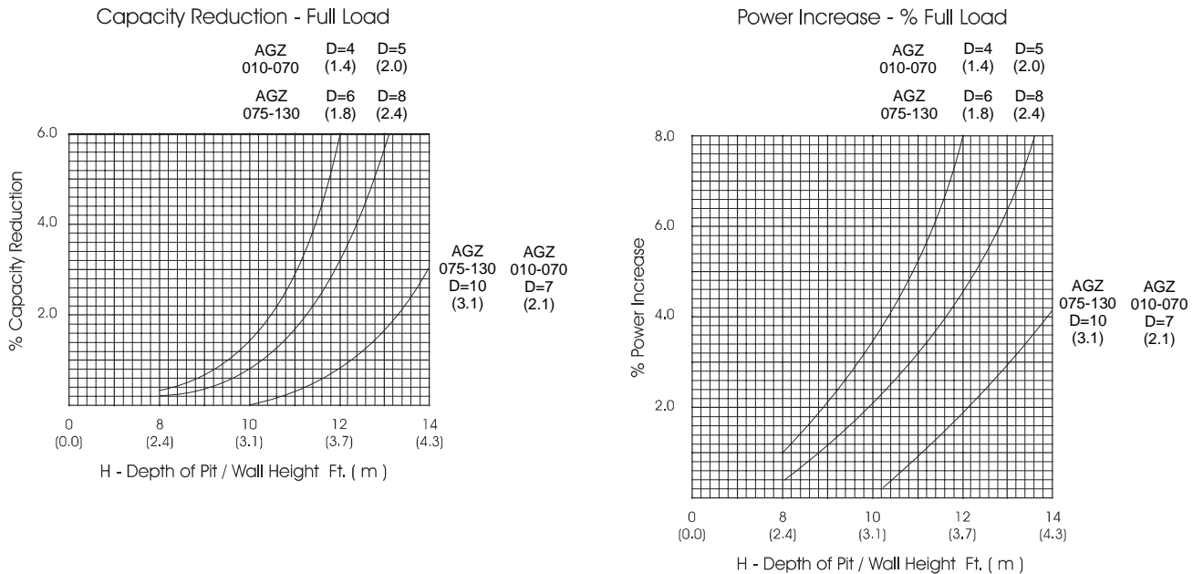
Figure 36, Adjustment Factor
