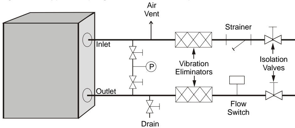
Figure 38, Typical Piping, Brazed-Plate Evaporator
