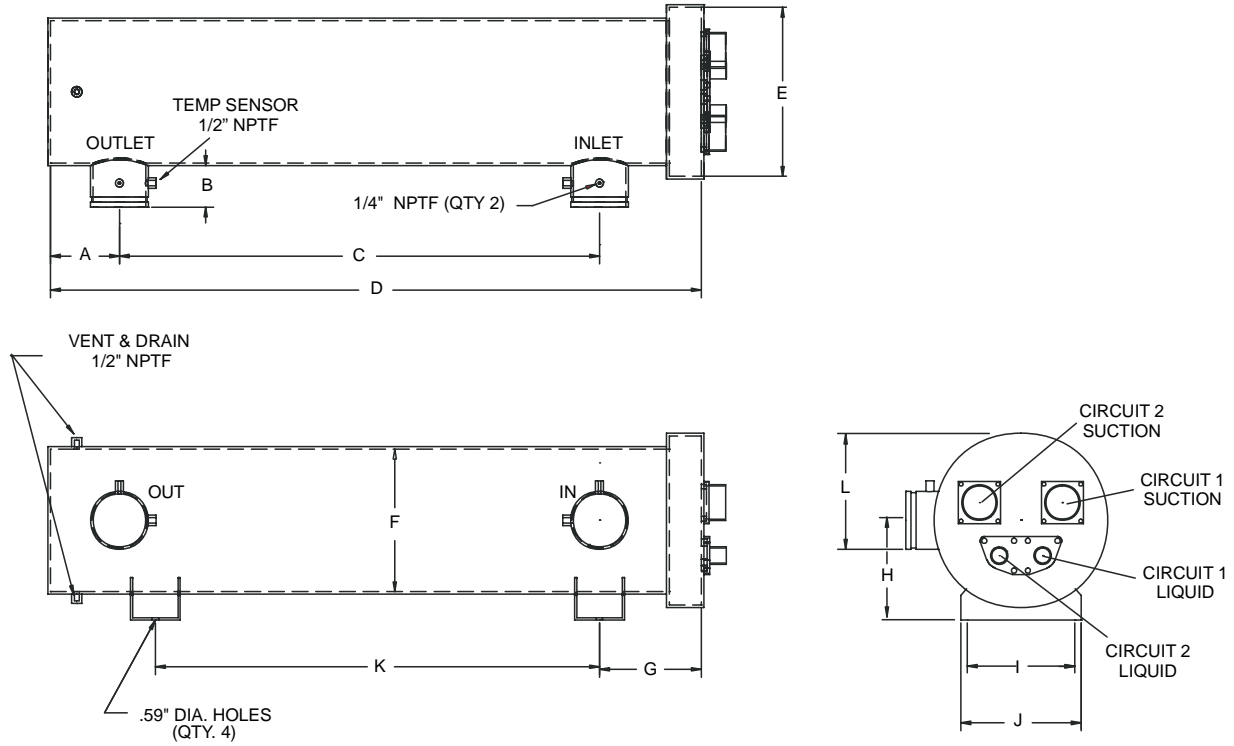
Figure 24, Remote Evaporators, AGZ 075BM/BB - 130BM/BB
