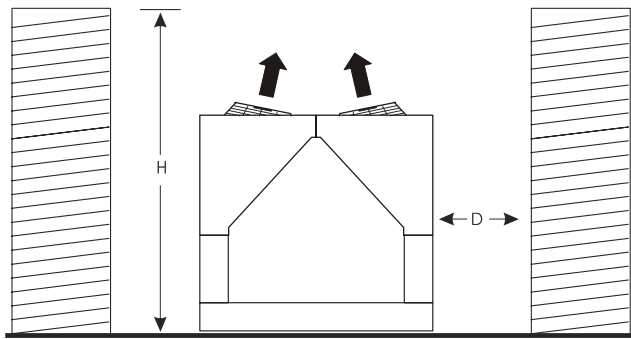
Figure 35, Pit Installation
