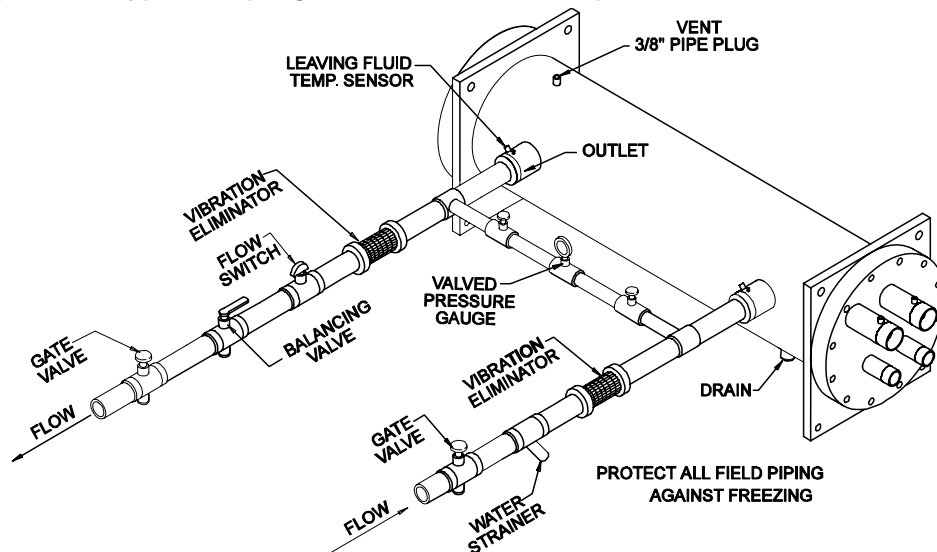
Figure 37, Typical Piping, Shell and Tube Evaporator
