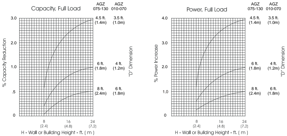
Figure 28, Adjustment Factors
