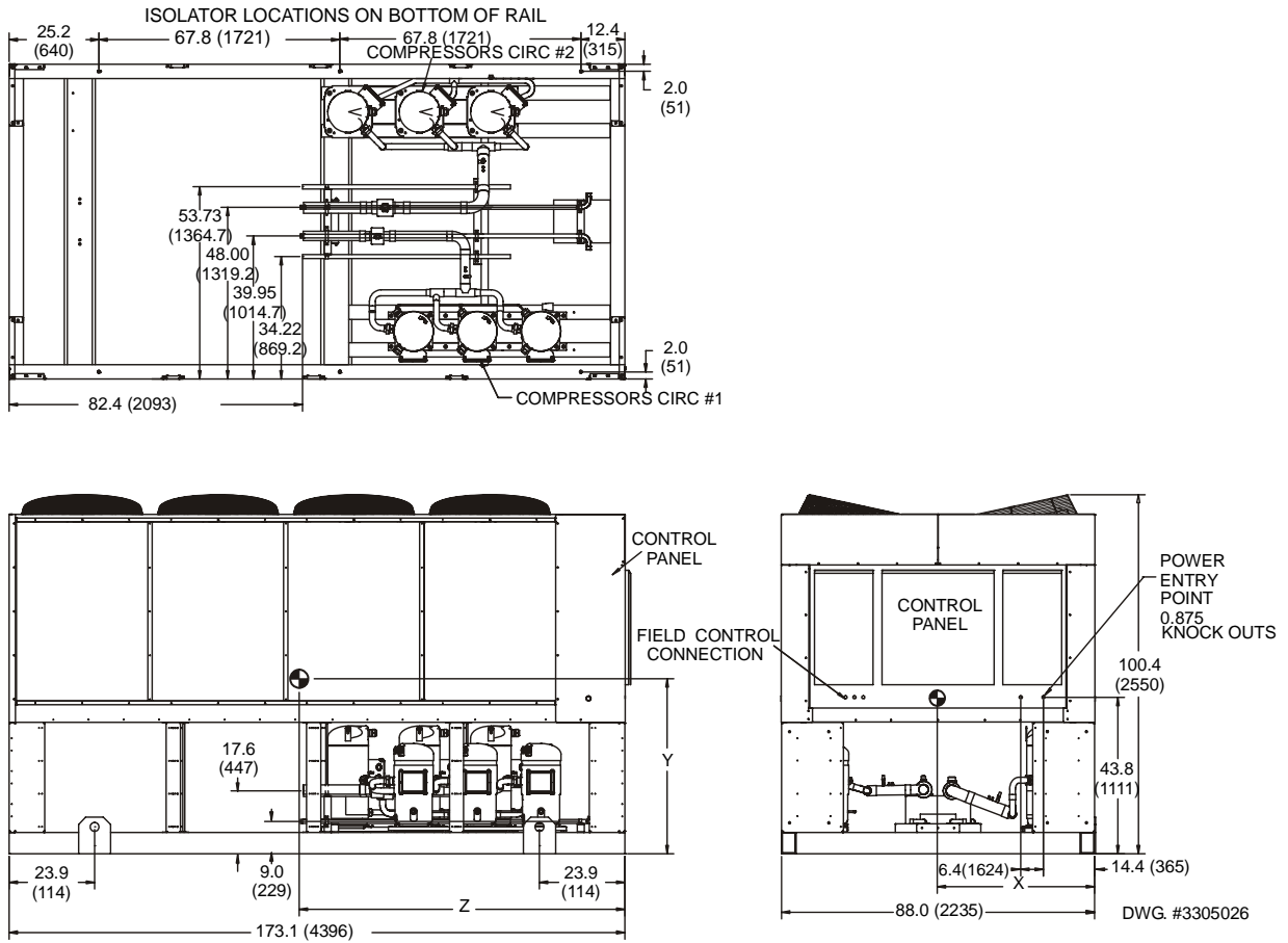
Figure 21, Dimensions, AGZ 100BM/BB - 130BM/BB, w/Remote Evaporator
