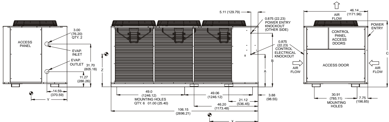
Figure 13, AGZ 020A through 034A
