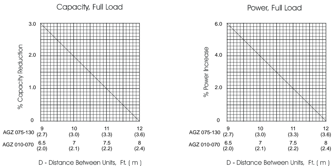
Figure 30, Adjustment Factor
