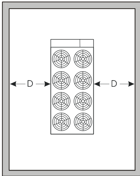
Figure 34, Wall Free Area vs Distance
