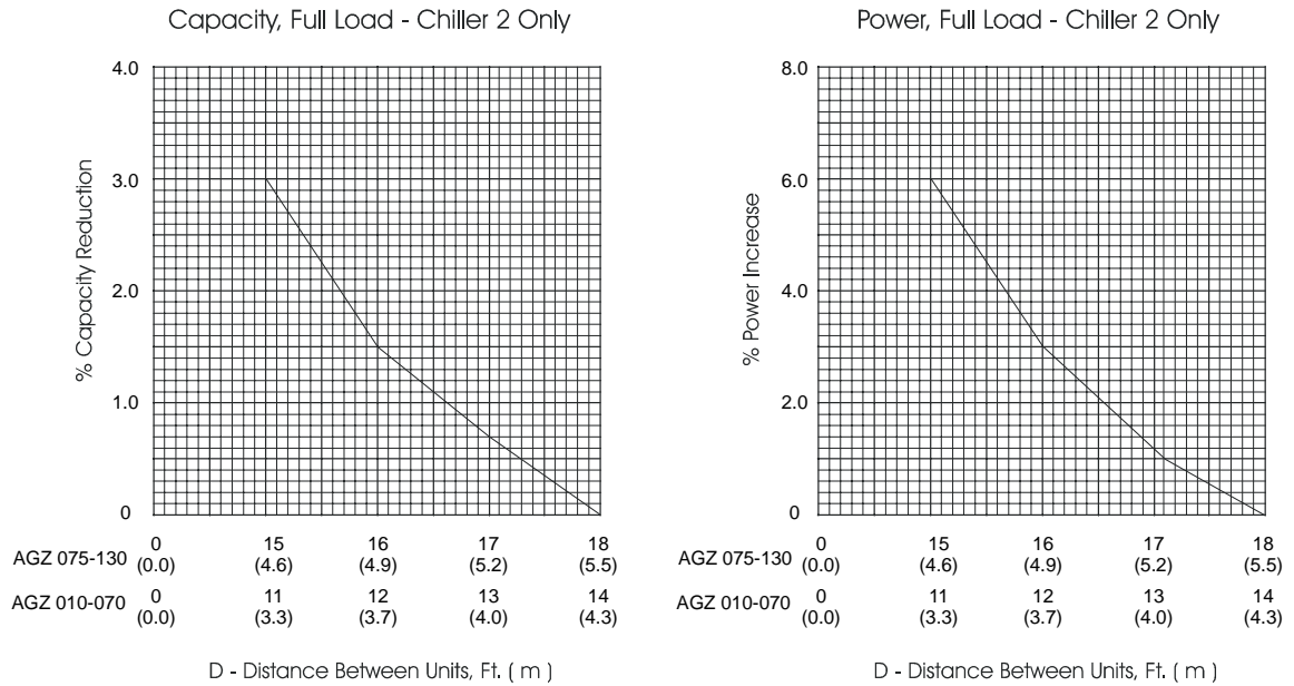
Figure 32, Adjustment Factor
