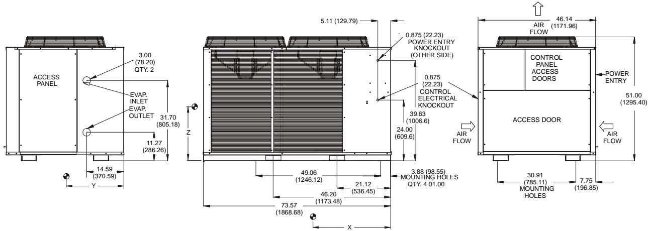
Figure 12, Dimensions AGZ 010A through 017A Packaged Chiller
