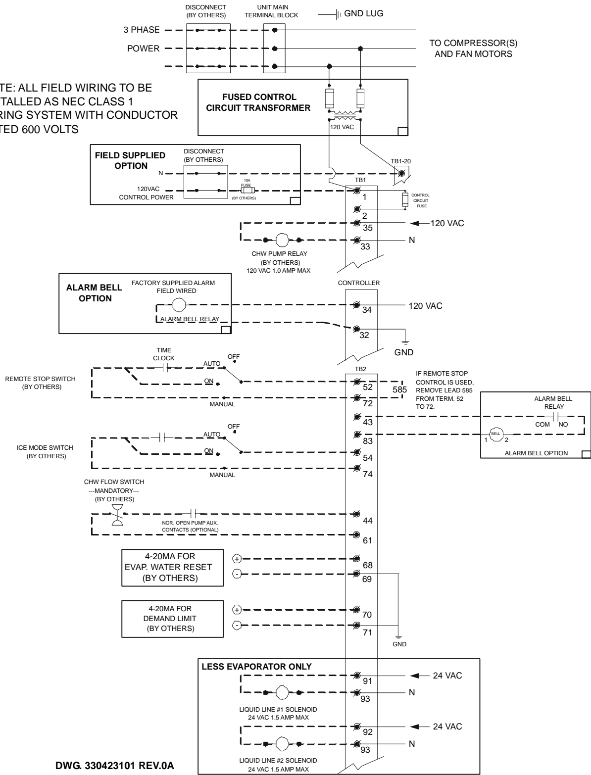
Figure 11, AGZ 026B – AGZ 130B, Typical Field Wiring
