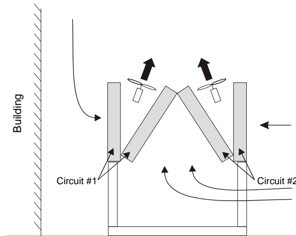
Figure 26, Coil and Fan Arrangement
