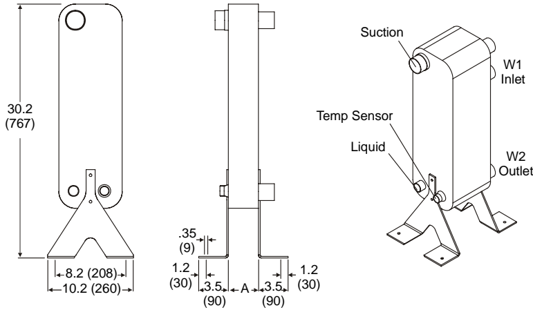
Figure 22, Remote Evaporators, for AGZ 010AM – 034AM
