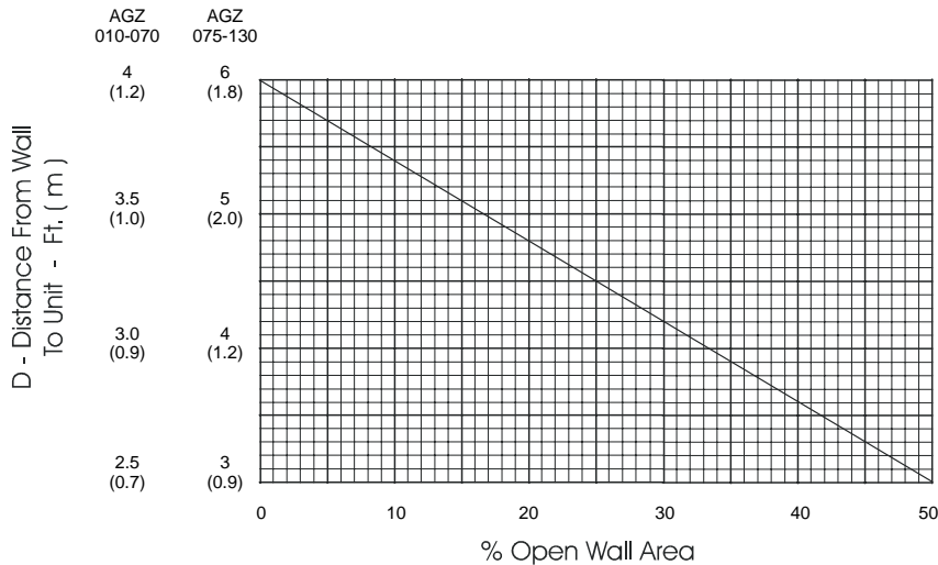
Figure 34, Wall Free Area vs Distance
