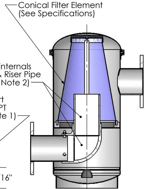
SECTION B-B
