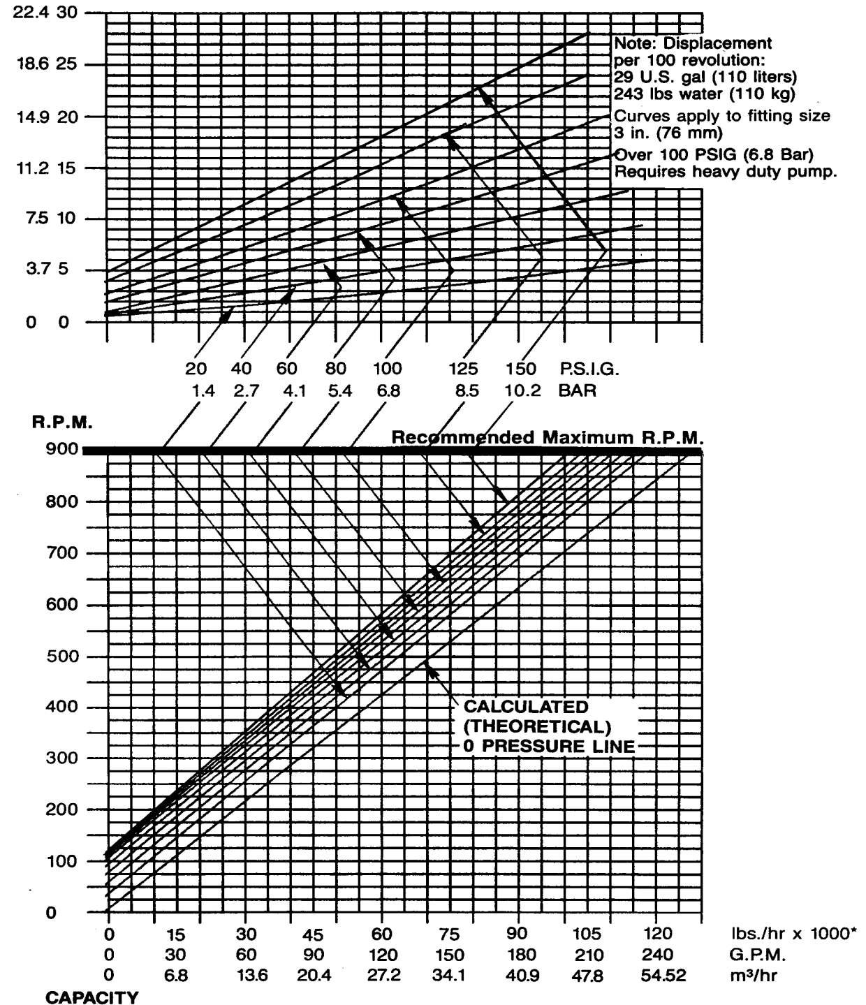
MODEL NO. 6 ROTARY PUMP CAPACITY CURVE
