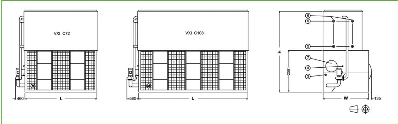
1. Drain ND xx; 2. Outlet connection NDxx; 3. Overflow NDxx; 4. Make up ND xx; 5. Inlet connection NDxx; 6. Vent NDxx; 7. Access door.
