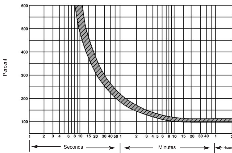
Trip Characteristics For Overload Relays
